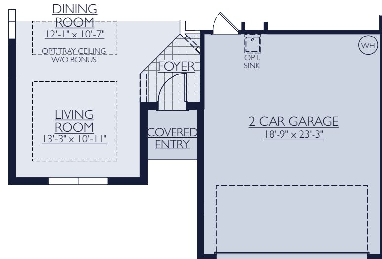
OPT 4' GARAGE EXTENSION
